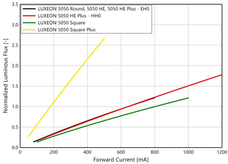
Figure 3b. Typical normalized light output vs. forward current for LUXEON 5050 - 6V, T_j=25^\circ\text{C}
