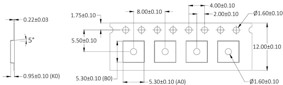
Figure 11b. Pocket Tape dimensions for LUXEON 5050 Round LES, LUXEON 5050 Square LES, LUXEON 5050 HE and LUXEON 5050 HE Plus
