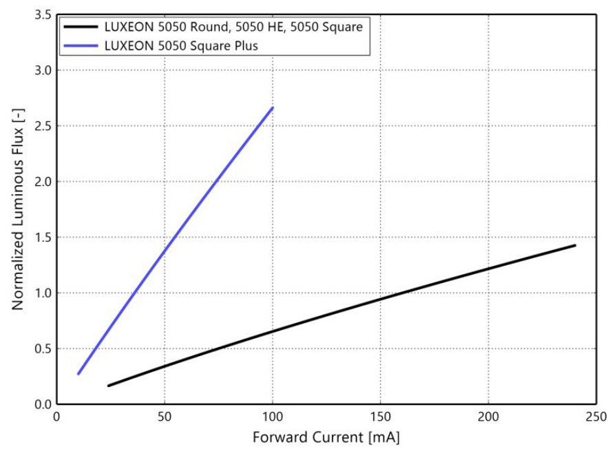
Figure 3a. Typical normalized light output vs. forward current for LUXEON 5050 - 24V/30V, T j =25°C
