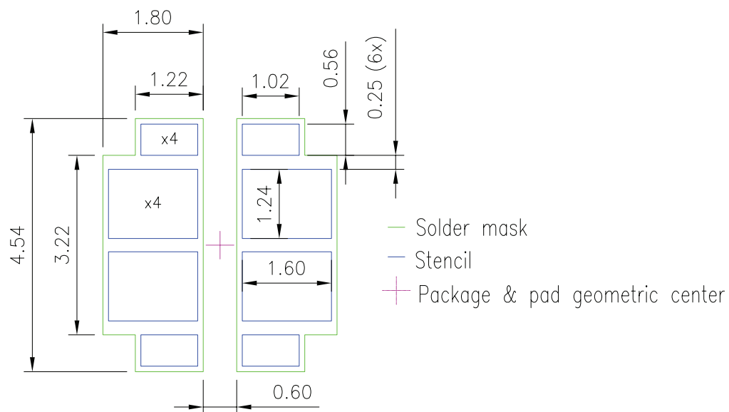
Figure 10. Recommended PCB solder pad layout for LUXEON 5050 Round LES, LUXEON 5050 Square LES, LUXEON 5050 HE and LUXEON 5050 HE Plus - HH0
