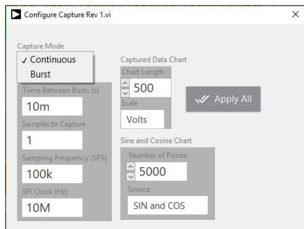
Figure 20. Configure Window
