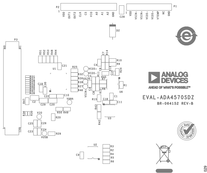
Figure 29. EVAL-ADA4570SDZ Silkscreen
