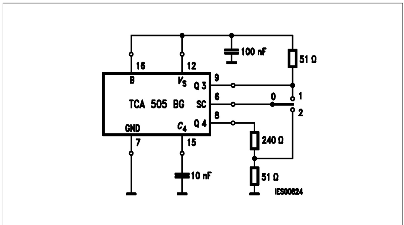
Figure 11 Test Circuit 2
