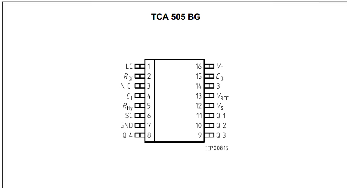
Figure 1 Pin Configurations (top view)
