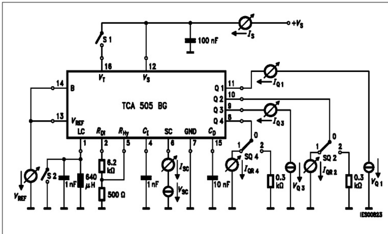
Figure 10 Test Circuit 1
