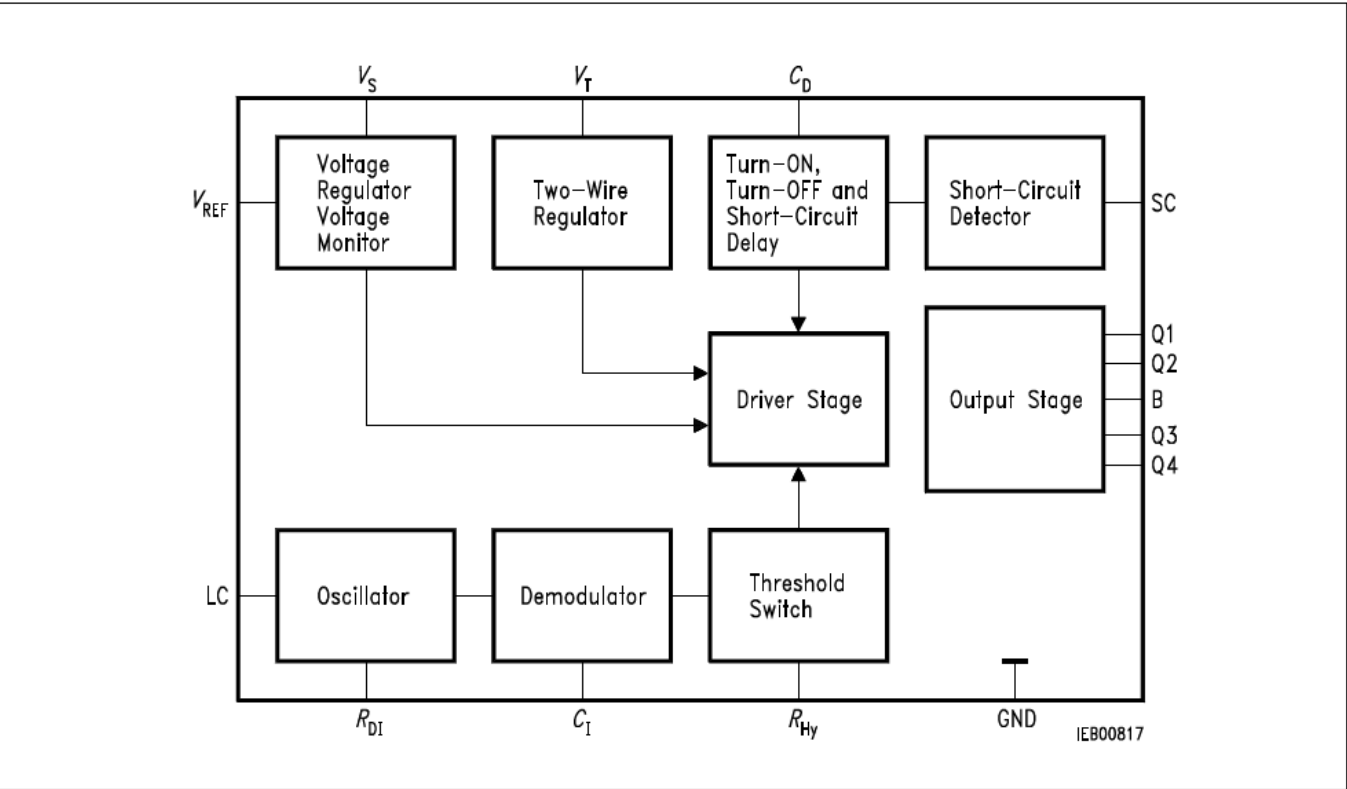
Figure 3 Block Diagram
