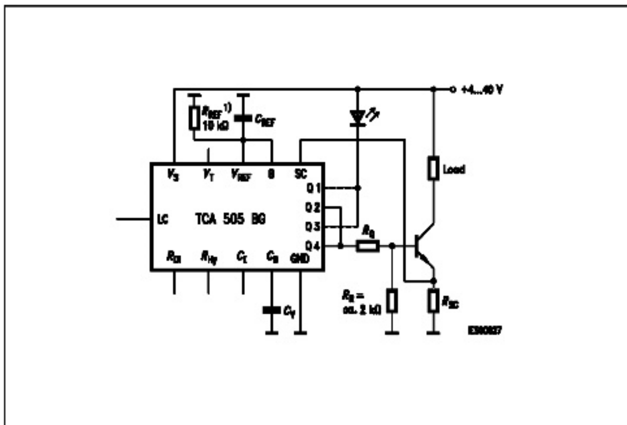
Output Circuitry (Use of pins V_{REF} , B, SC, Q1 through Q4, C_D )
