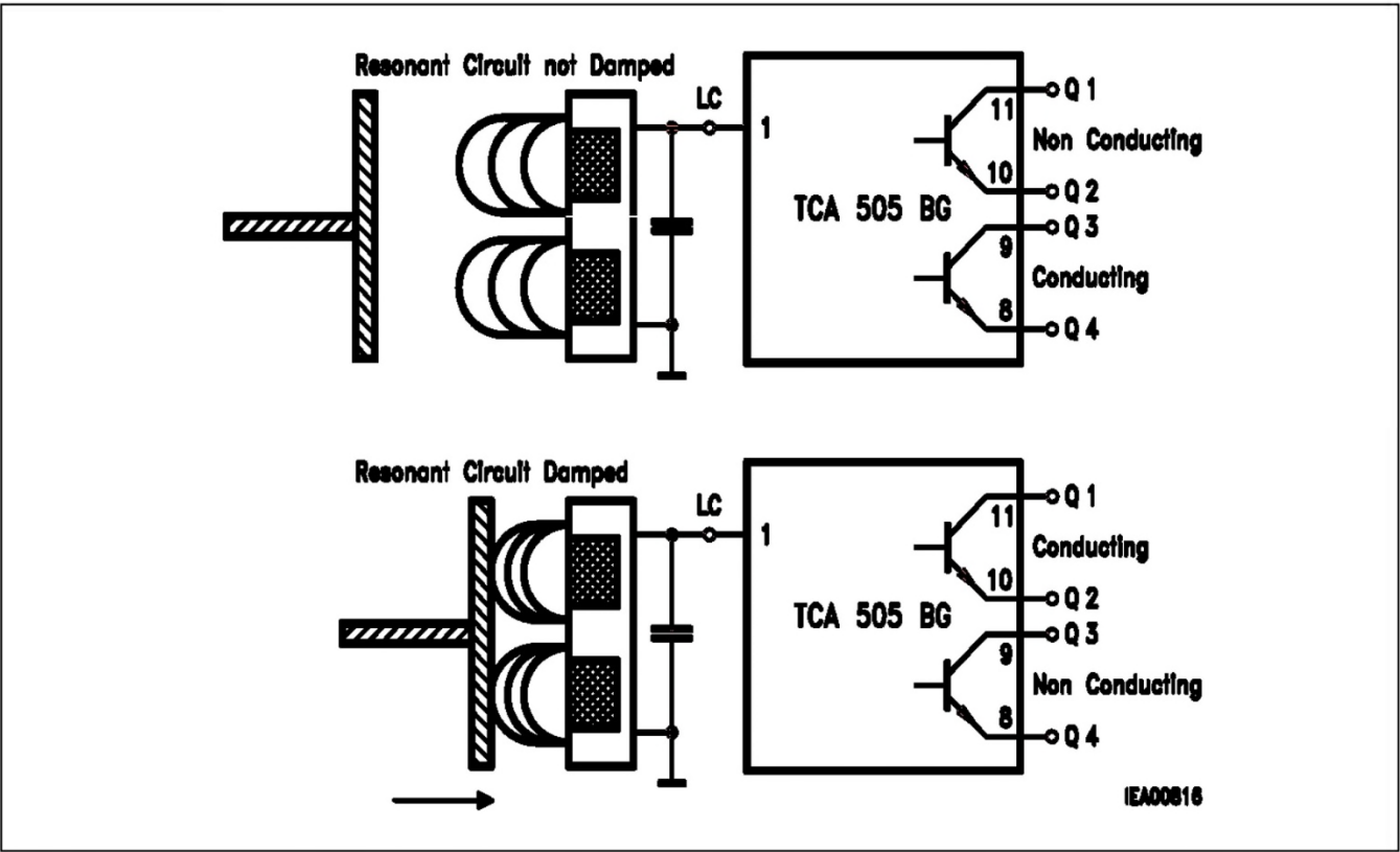
Figure 2 Operation Schematic
