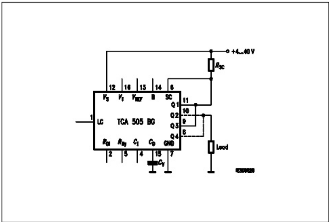
Figure 15 Application Circuit 4
