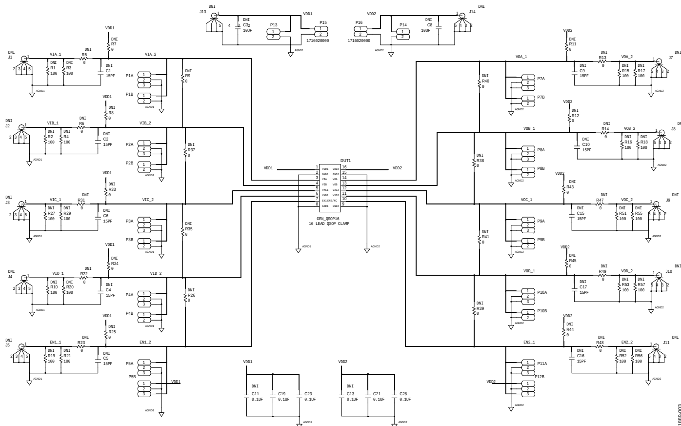
Figure 4. EVAL-ADuM1441EBZ Schematic
