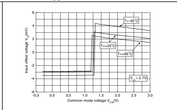
Figure 2. V_{IO} versus V_{ICM} and temperature at V_{CC} = 2.7\text{ V}
