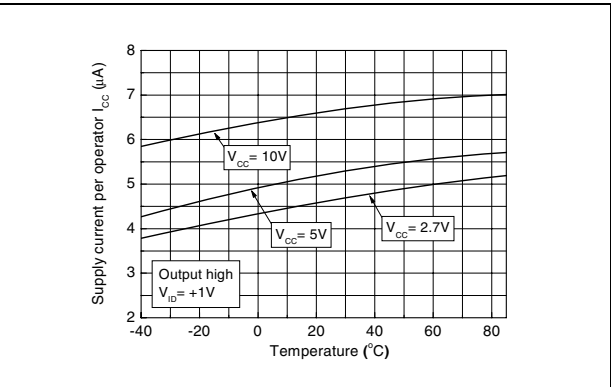
Figure 12. Supply current ( I_{CC} ) versus temperature
