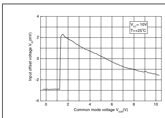
Figure 5. V_{IO} versus V_{ICM} at V_{CC} = 10\text{ V}
