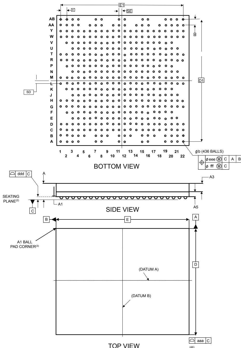
Figure 67. TFBGA436 - Outline
