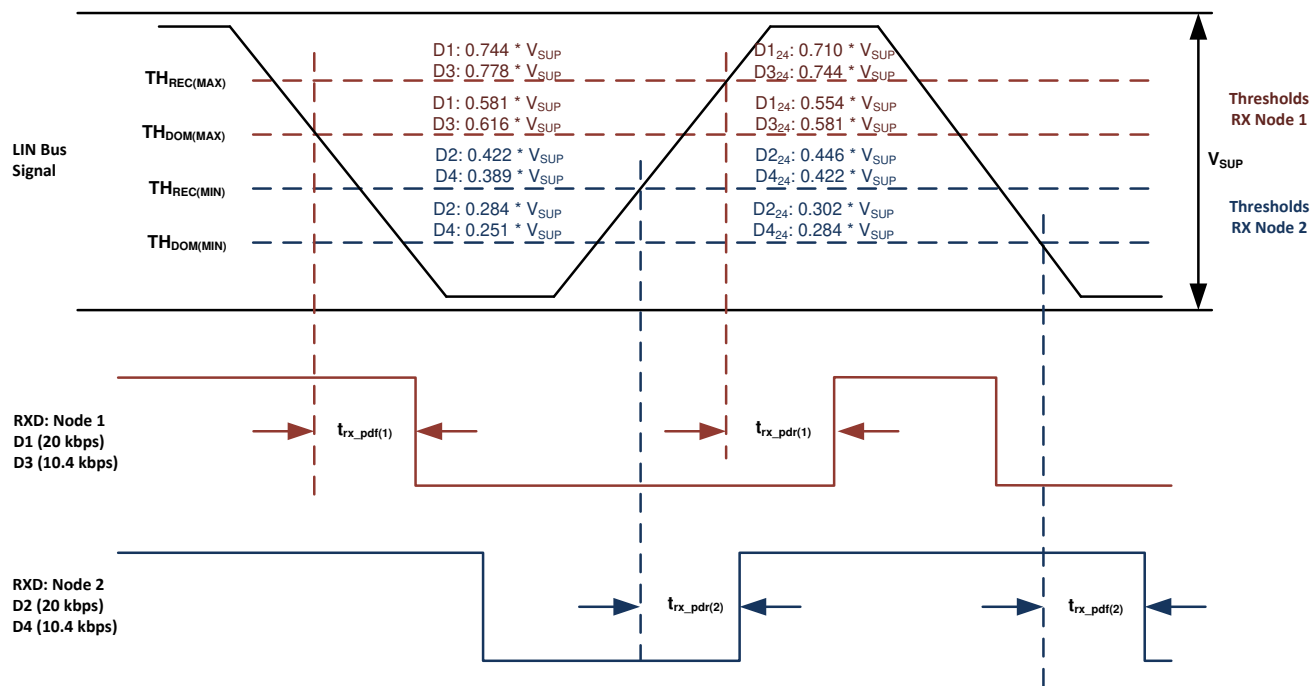
Figure 8-13. Propagation Delay
