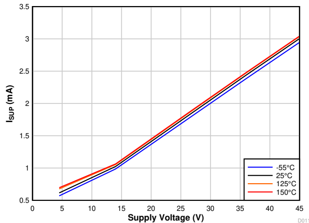
Figure 7-3. I_{SUP} Dominant vs V_{SUP} and Temperature
