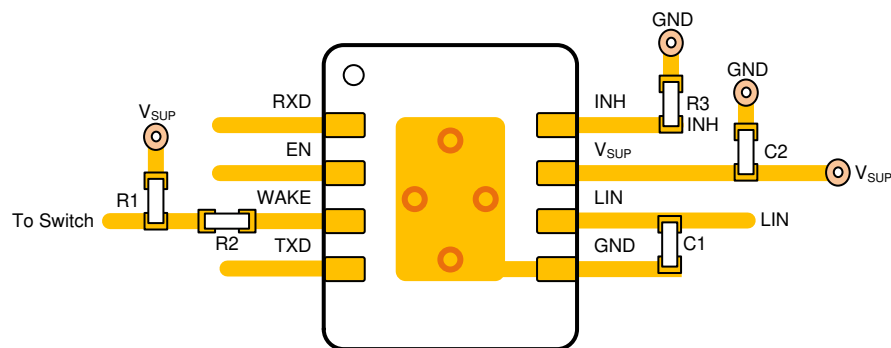
Figure 10-4. Layout Example
