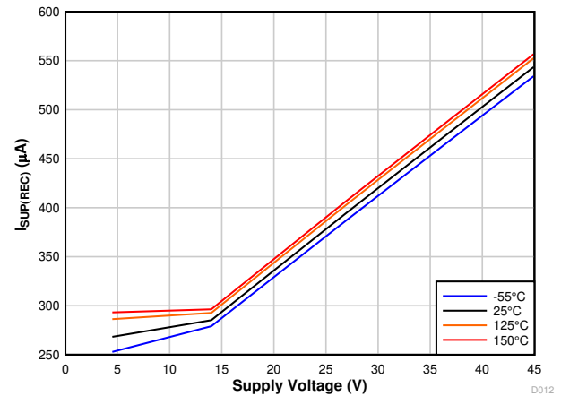
Figure 7-4. I_{SUP} Recessive vs V_{SUP} and Temperature
