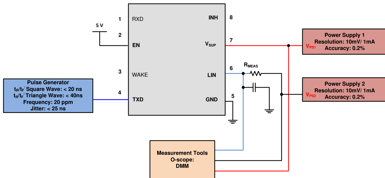
Figure 8-10. Test Circuit Slope Control and Duty Cycle Param 27, 28, 29, 30 , 72, 73, 74, 75
