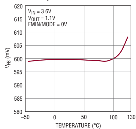
LTC3620 Feedback Voltage vs Temperature
