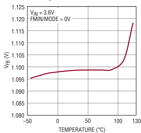
LTC3620-1 Feedback Voltage vs Temperature
