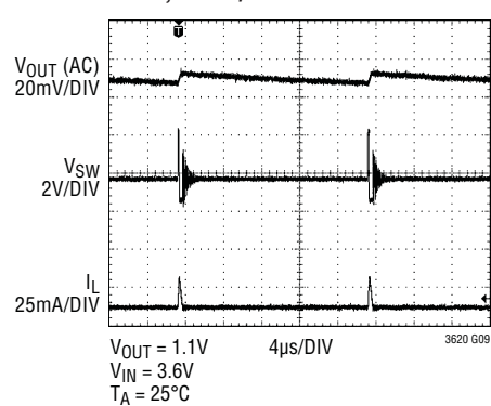
Switching Waveforms at 250 \mu\text{A} Load, FMIN/MODE = 0V
