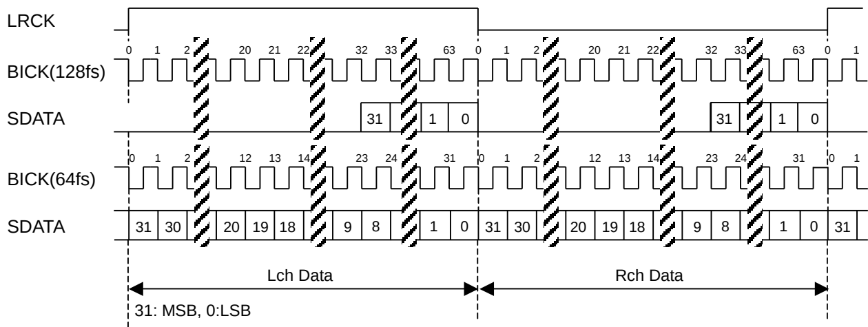
Figure 13. Mode 5 Timing
