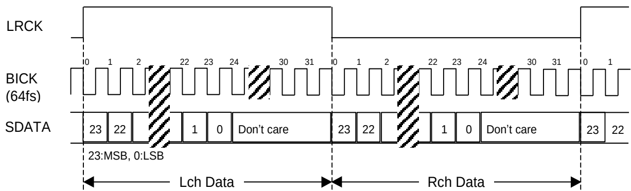
Figure 11. Mode 2 Timing
