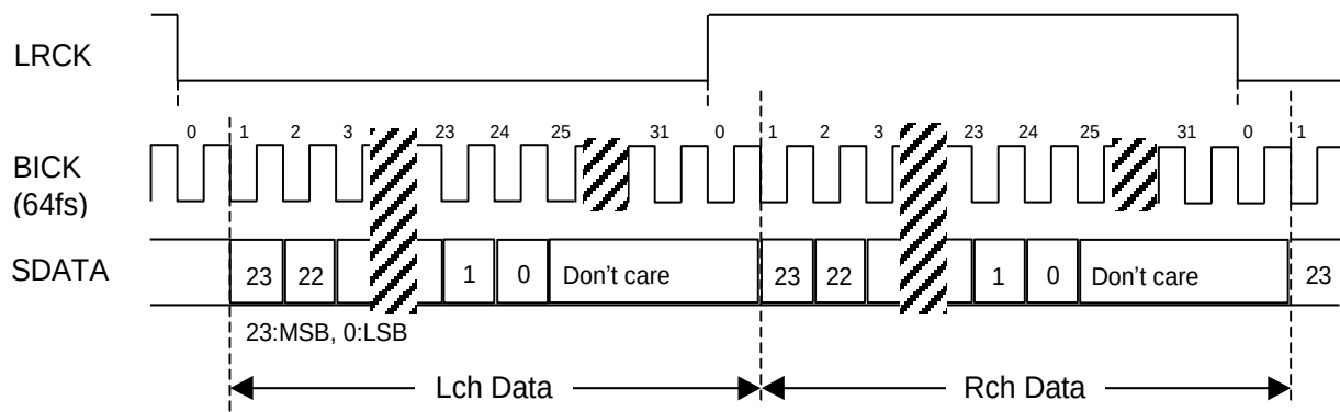
Figure 12. Mode 3 Timing
