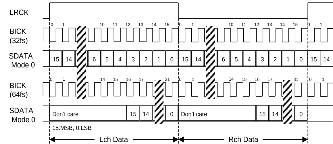
Figure 9. Mode 0 Timing
