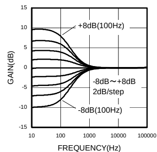
Fig.9 Bass Gain - Frequency (BD3401KS2)
