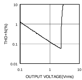
Fig.18 Total Harmonic Distortion ratio - Output Voltage (PB)
