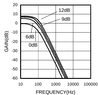
Fig.15 Subwoofer Gain - Frequency (BD3401KS2)
