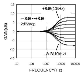
Fig.12 Treble Gain - Frequency
