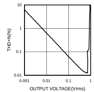
Fig.21 Total Harmonic Distortion ratio – Output Voltage (REC)
