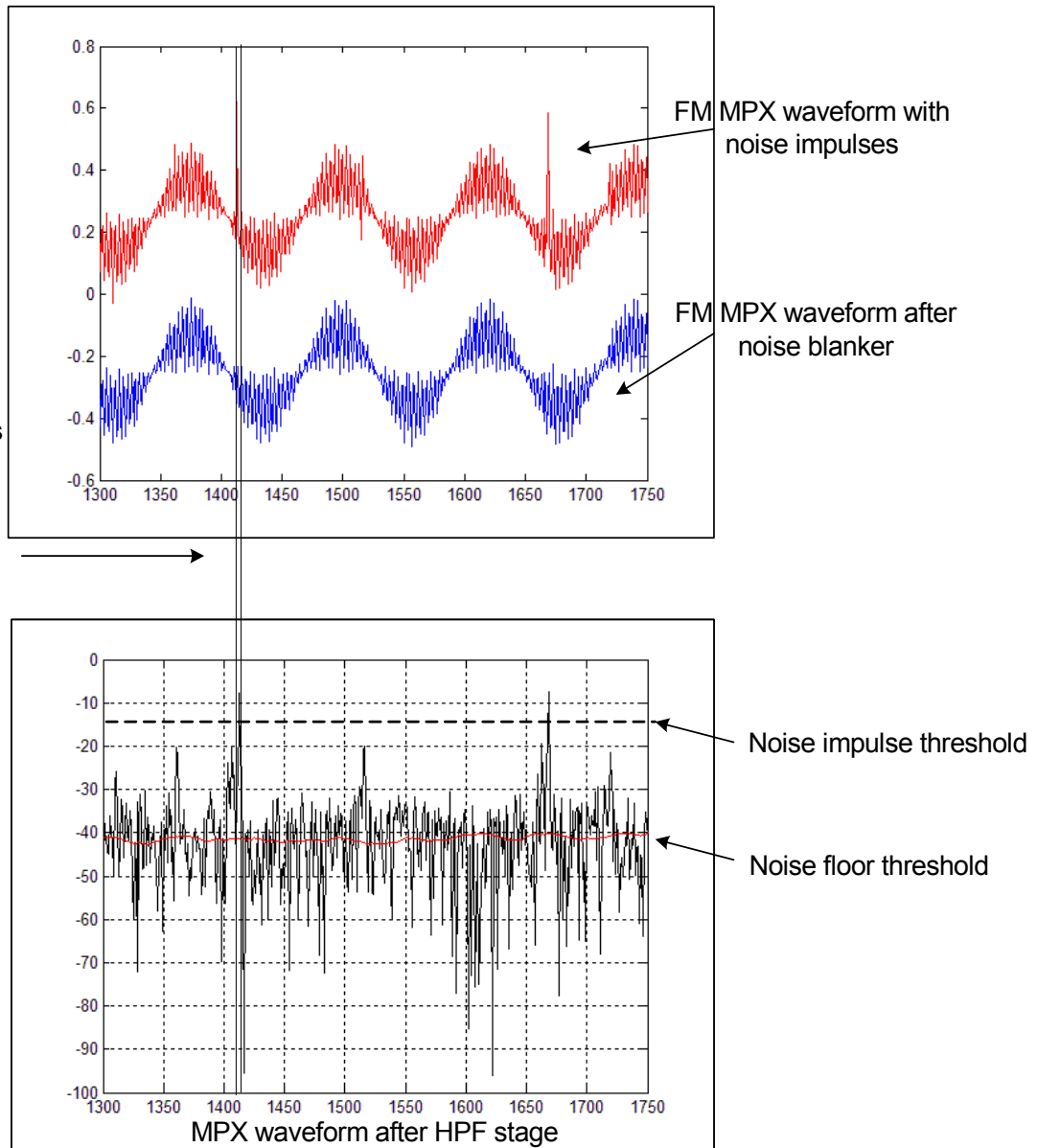
Figure 19. Illustration of FM Noise Blanker Property Settings for Proper Detection of Noise Impulses (FM MPX waveforms are offset vertically for illustration purposes)
