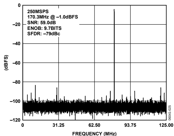
Figure 15. AD9211-250 64k Point Single-Tone FFT; 250 MSPS, 170.3 MHz
