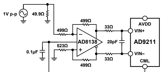
Figure 39. Differential Input Configuration Using the AD8138
