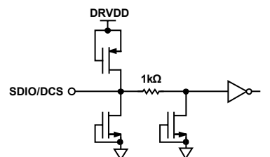
Figure 38. Equivalent SDIO/DCS Input Circuit
