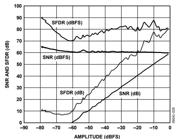
Figure 17. AD9211-250 SNR/SFDR vs. Input Amplitude; 250 MSPS, 170.3 MHz
