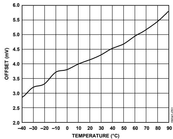
Figure 32. Offset vs. Temperature
