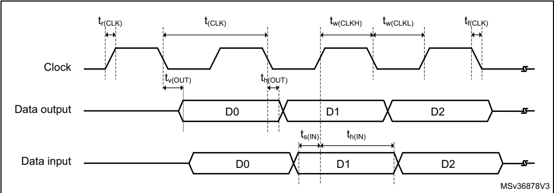
Figure 67. OCTOSPI timing diagram - SDR mode
