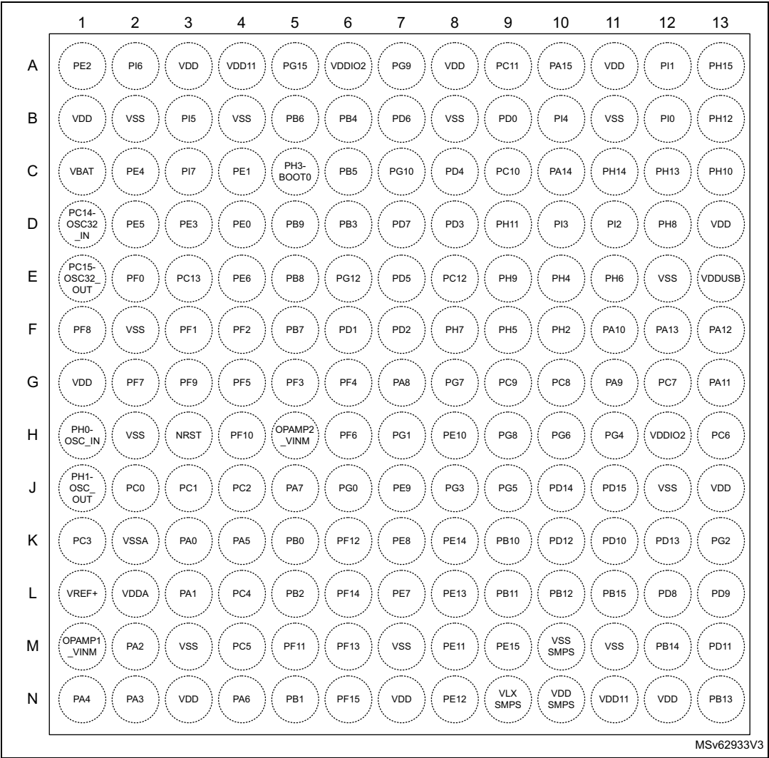
Figure 17. TFBGA169_SMPS ballout
