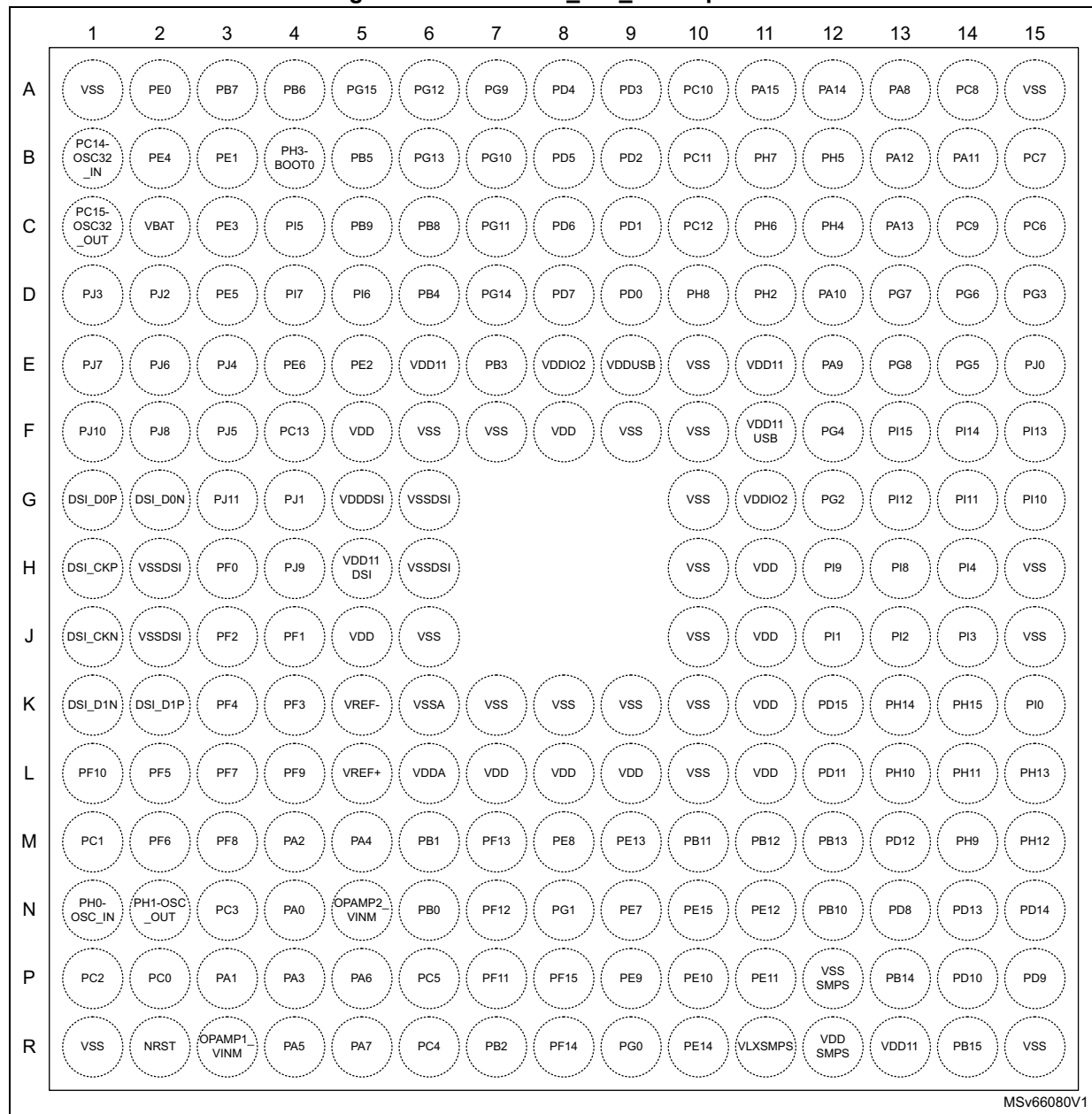
Figure 20. TFBGA216_DSI_SMPS pinout
