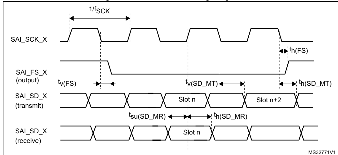
Figure 81. SAI master timing diagram
