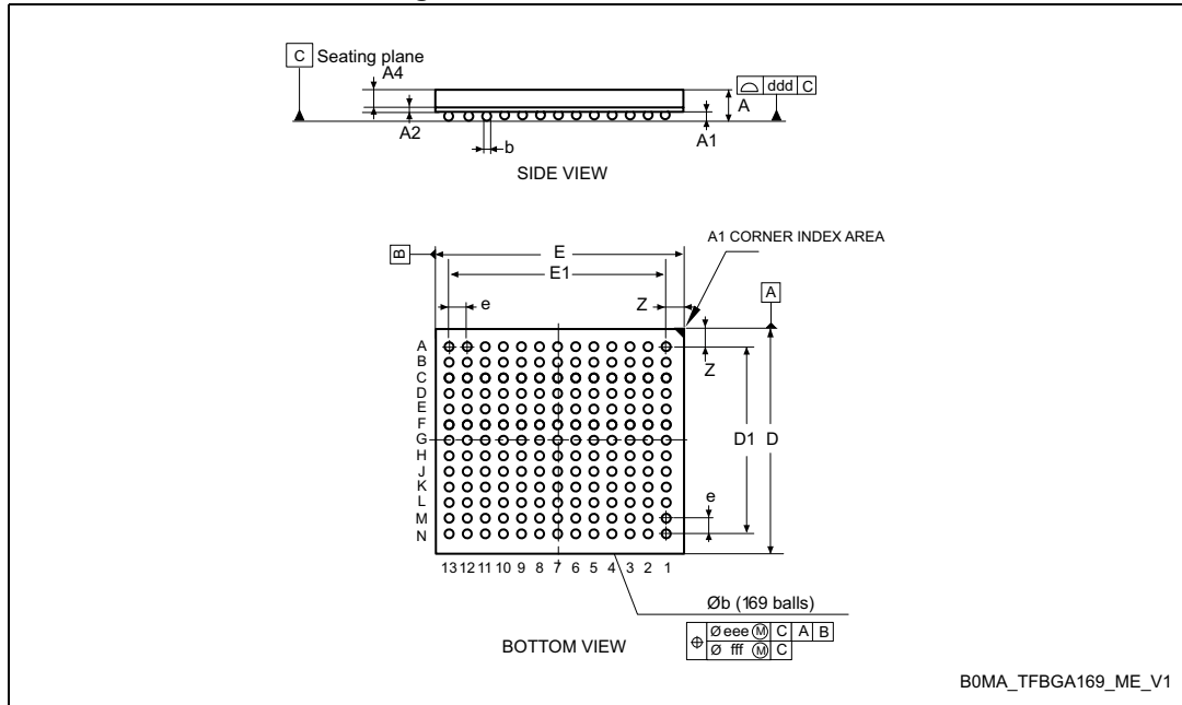
Figure 99. TFBGA169 - Outline
