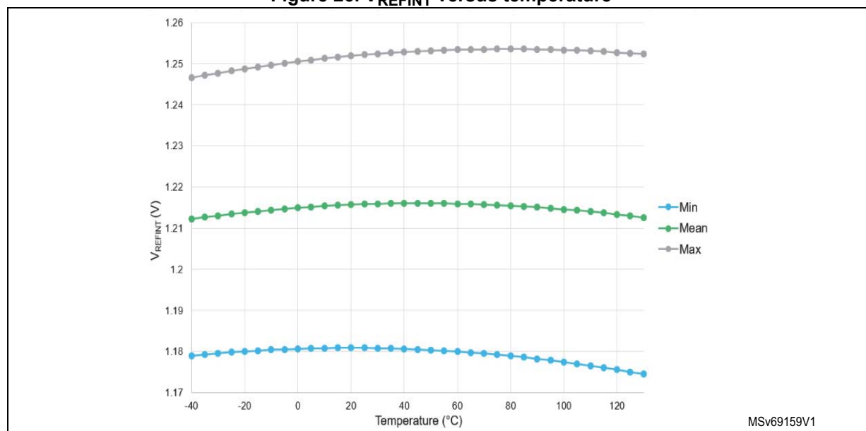
Figure 26. V_{REFINT} versus temperature
