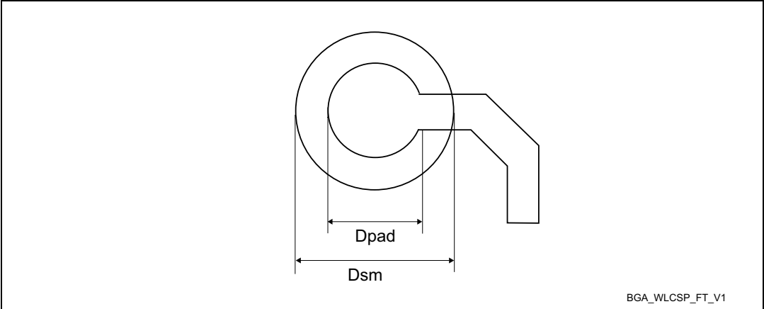
Figure 98. WLCSP150 - Recommended footprint
