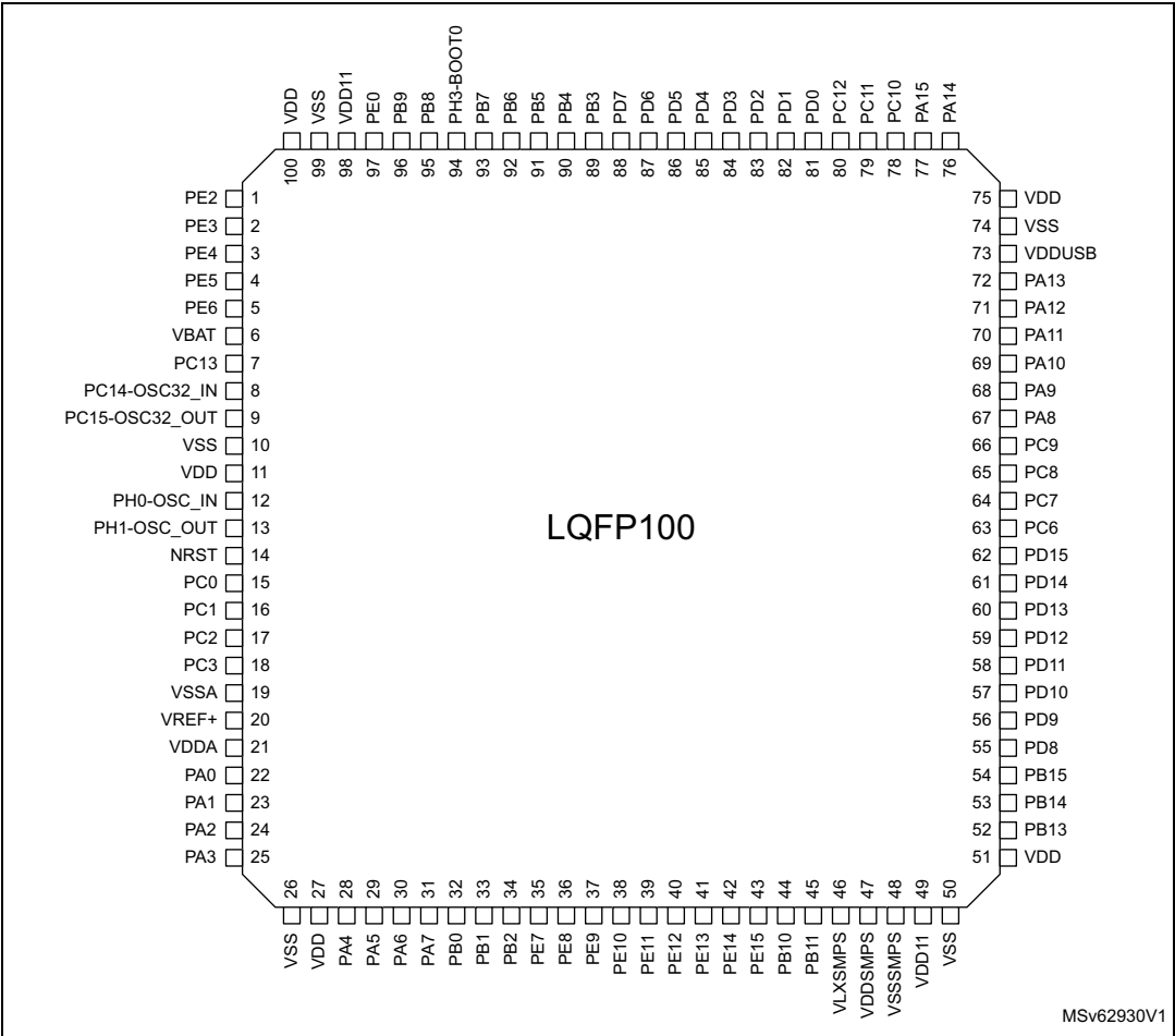
Figure 9. LQFP100_SMPS pinout
