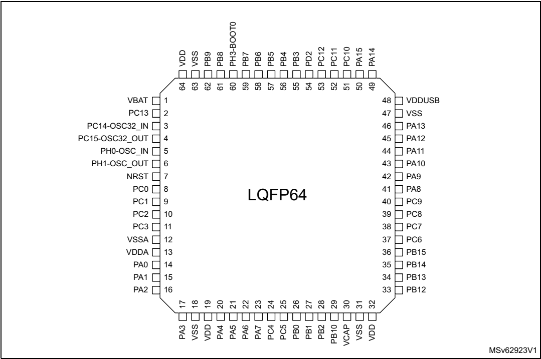
Figure 8. LQFP64 pinout
