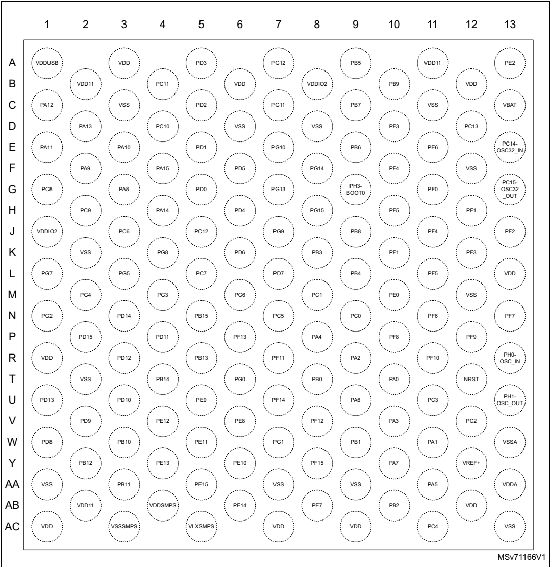
Figure 15. WLCSP150_SMPS ballout
