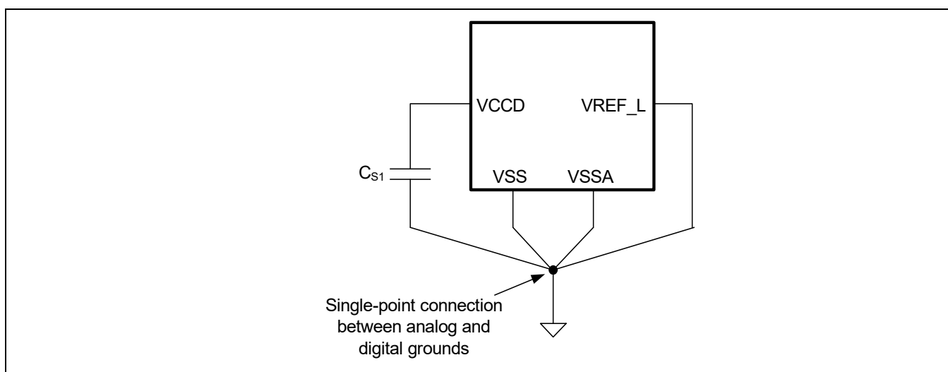
Figure 26-2 Smoothing capacitor
