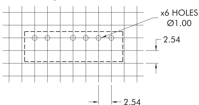
7 Pin SIP Package
