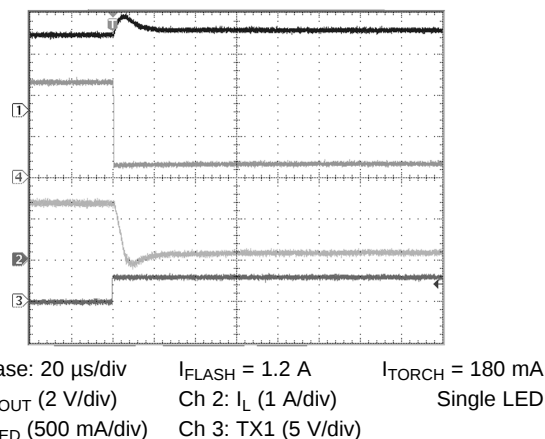
Figure 56. TX1 Interrupt Operation, TX1 Rising
