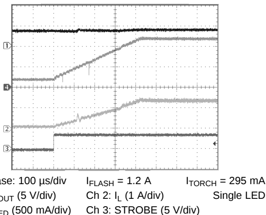
Figure 55. Torch Mode to Flash Mode Transition
