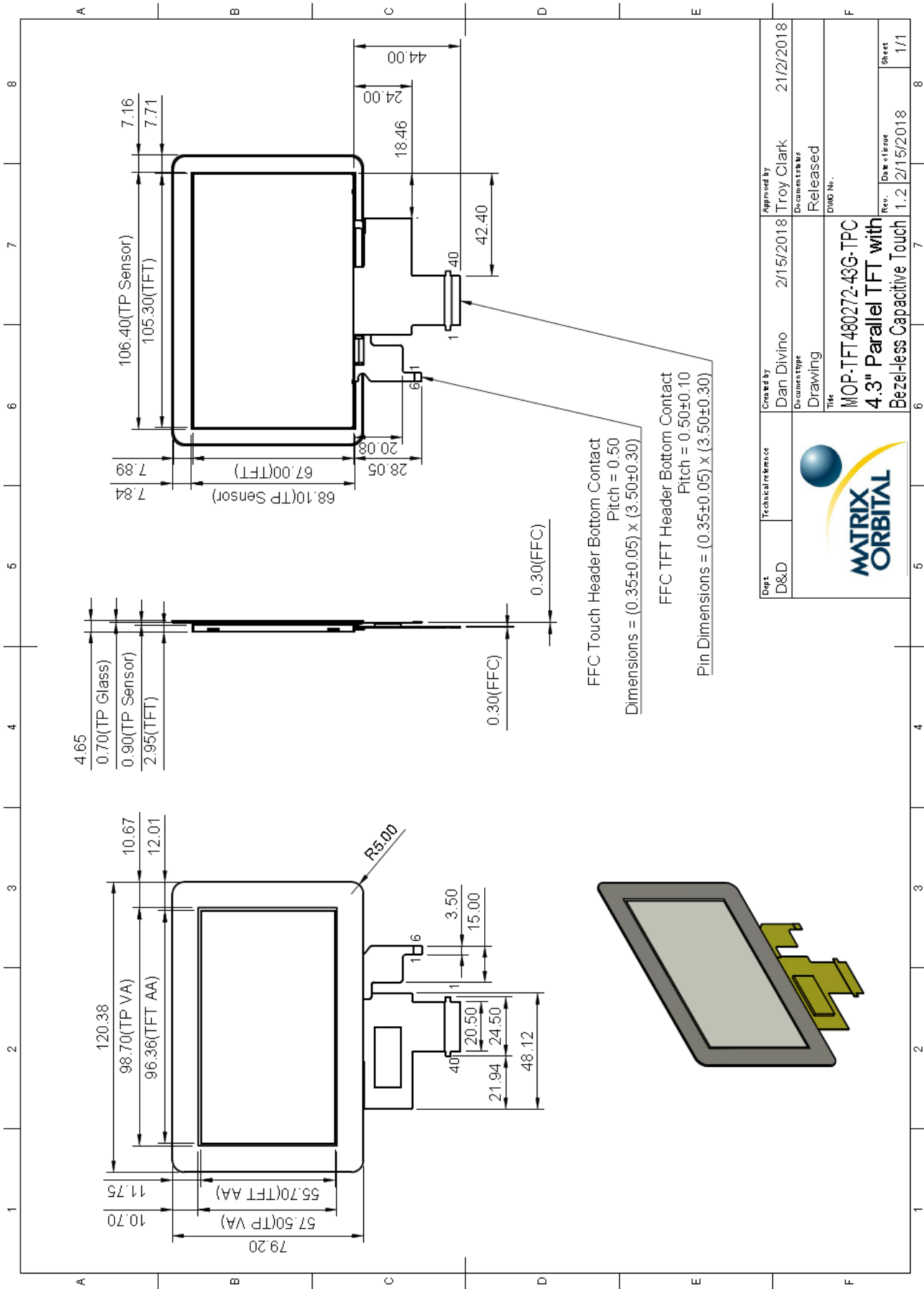
Figure 1: MOP-TFT480272-43G-BLM-TPC Drawing
