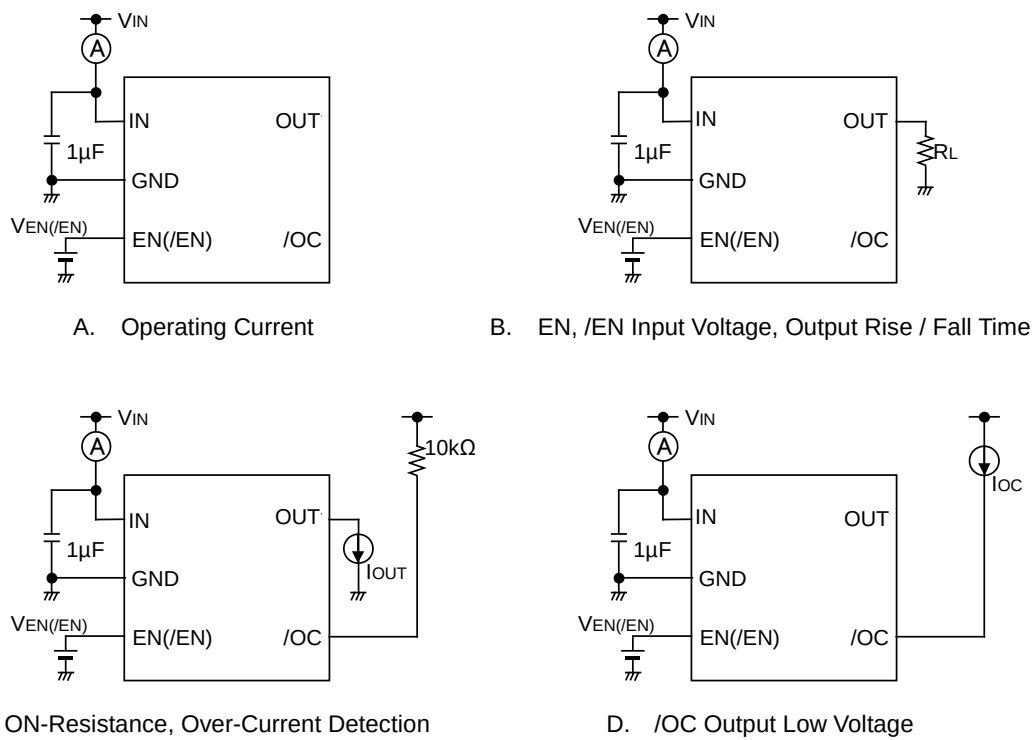
Figure 1. Measurement Circuit
