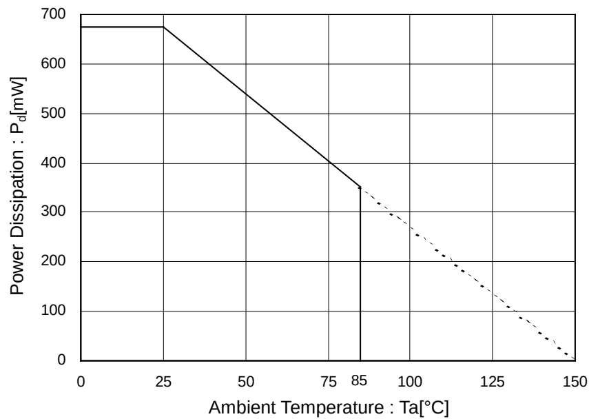
Figure 42. Power Dissipation Curve (Pd-Ta Curve)
