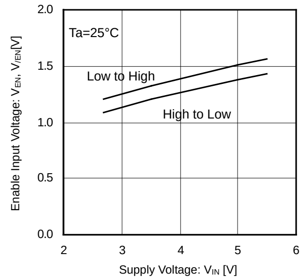
Figure 8. EN, /EN Input Voltage vs Supply Voltage ( V_{ENH} , V_{ENL} , V_{/ENH} , V_{/ENL} )
