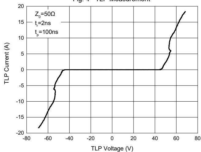
Fig. 4 - TLP Measurement
