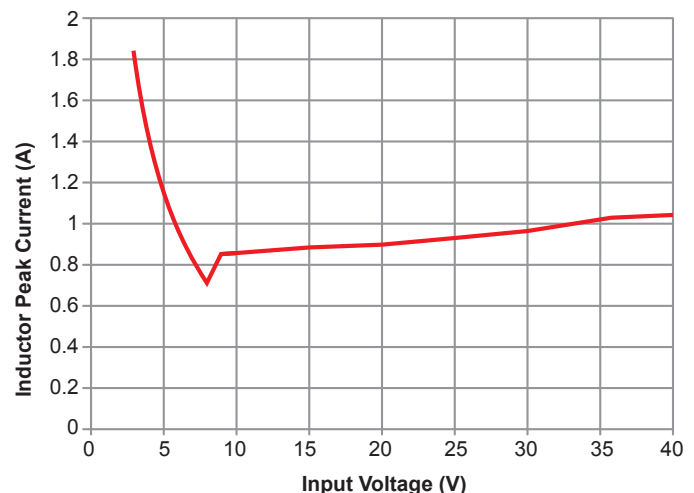
Figure 8: Typical Peak Inductor Current versus Input Voltage for 0.8 A Output Current and 10 \mu\text{H} Inductor
