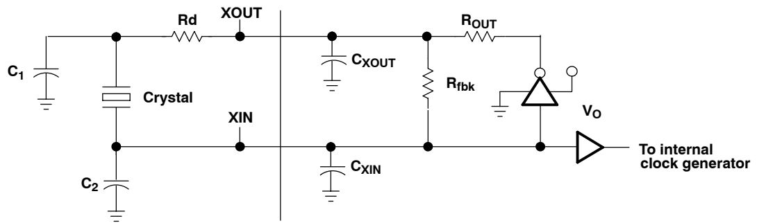
Figure 16. On-Chip Oscillator Circuit
