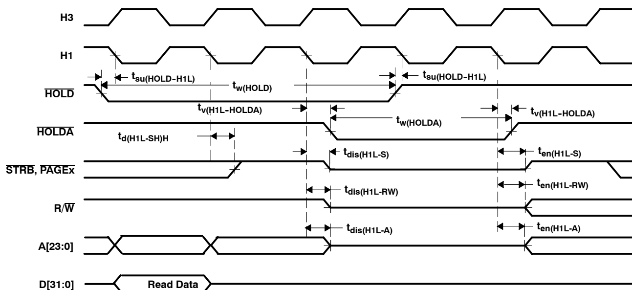
Figure 34. Timing for \overline{\text{HOLD}}/\overline{\text{HOLDA}} (After Read)
