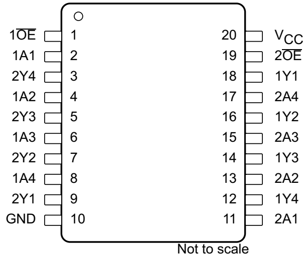
Figure 5-2. DB, DGV, DW, N, NS, and PW Packages 20-Pin SSOP, TVSOP, SOIC, PDIP, SO, and TSSOP Front View
