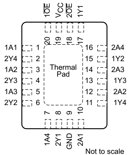
Figure 5-4. RWP Package 20-Pin X1QFN Top View
