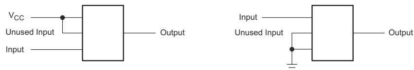
Figure 11-1. Layout Diagram
