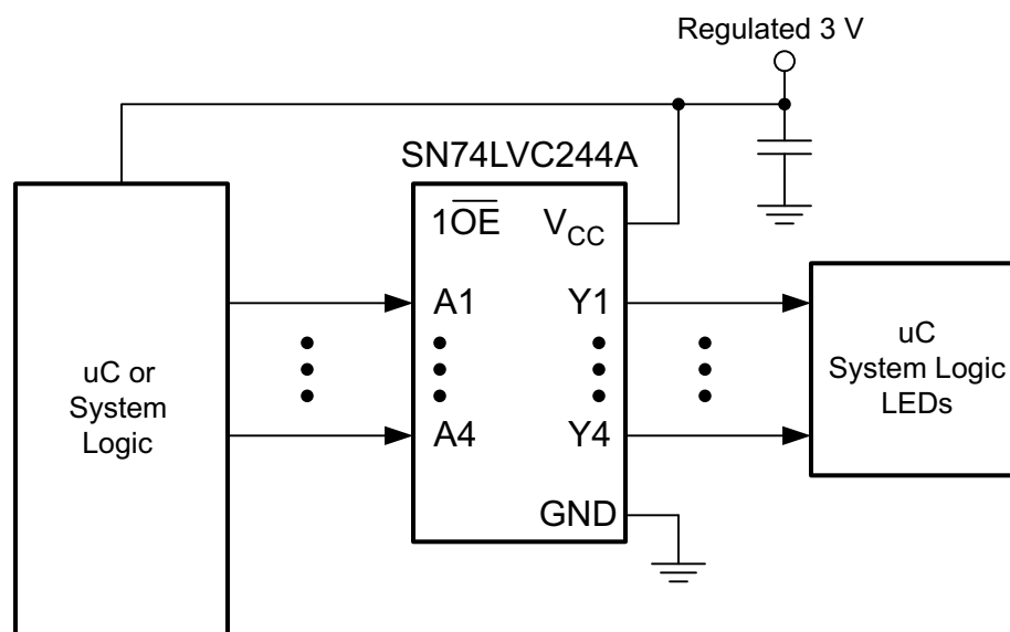
Figure 9-1. Application Schematic
