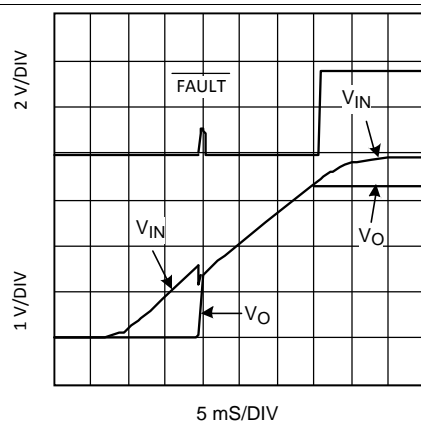
Figure 11. Power-Up Response
