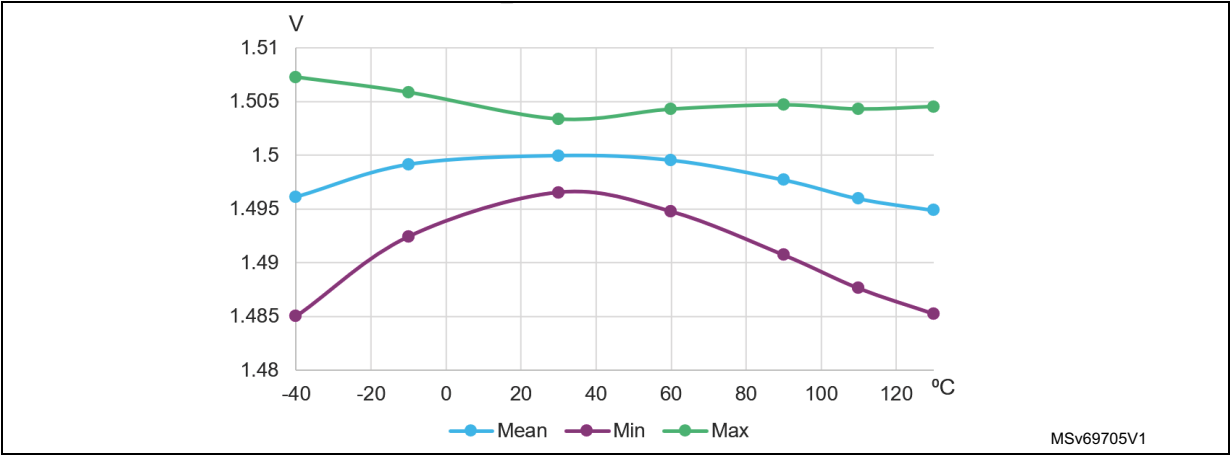
Figure 33. V_{REFBUF\_OUT} versus temperature (VRS = 000)
