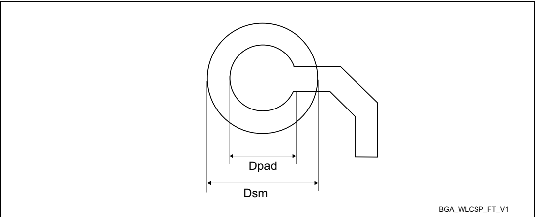
Figure 90. WLCSP208 - Recommended footprint
