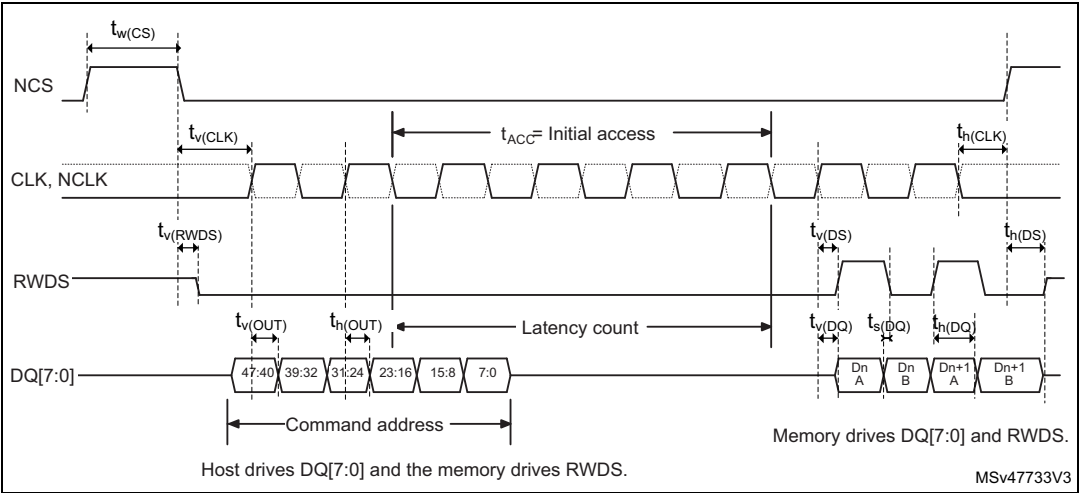
Figure 63. OCTOSPI HyperBus read
