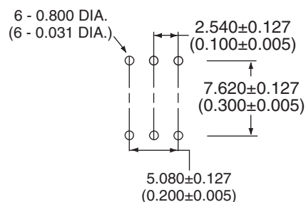
PCB Hole Pattern
