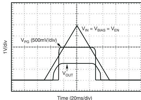
Figure 5-37. Turnon Response
