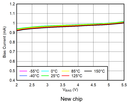
Figure 5-25. BIAS Pin Current vs V_{\text{BIAS}} and Temperature ( T_J )
