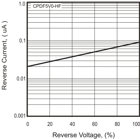
Fig.2-3 - Reverse Characteristics
