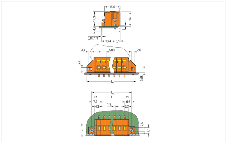
Dimensions in mm L = (pole no. x pin spacing) + 3 mm L1 = L + 5.8 mm L2 = L1 + 6.4 mm for plate thickness up to 1.5 mm
