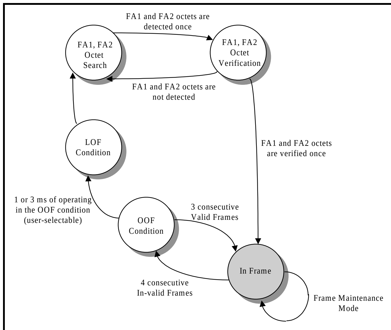
FIGURE 181. THE STATE MACHINE DIAGRAM FOR THE RECEIVE E3 FRAMER E3 FRAME ACQUISITION/MAINTENANCE ALGORITHM
