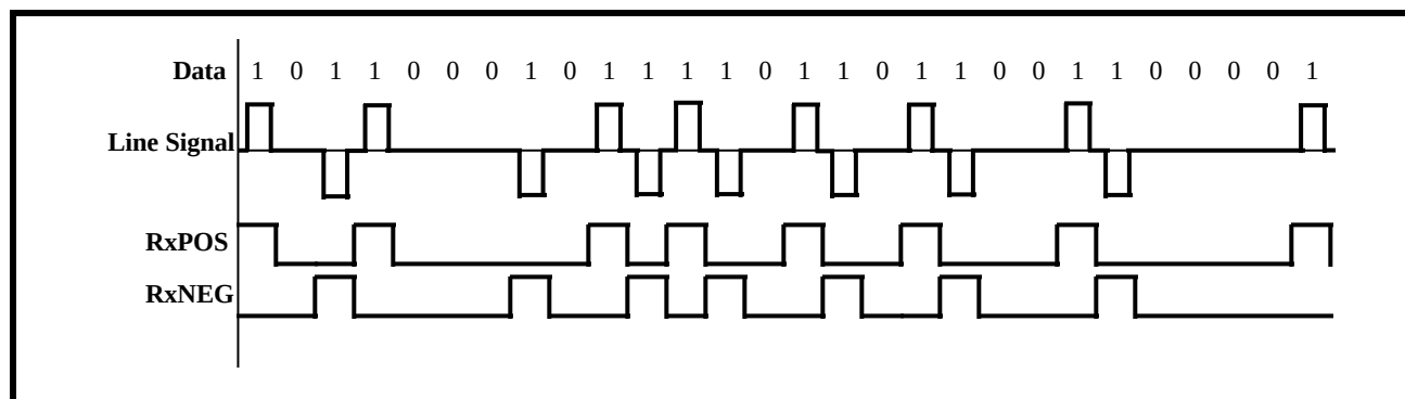
FIGURE 63. AMI LINE CODE
