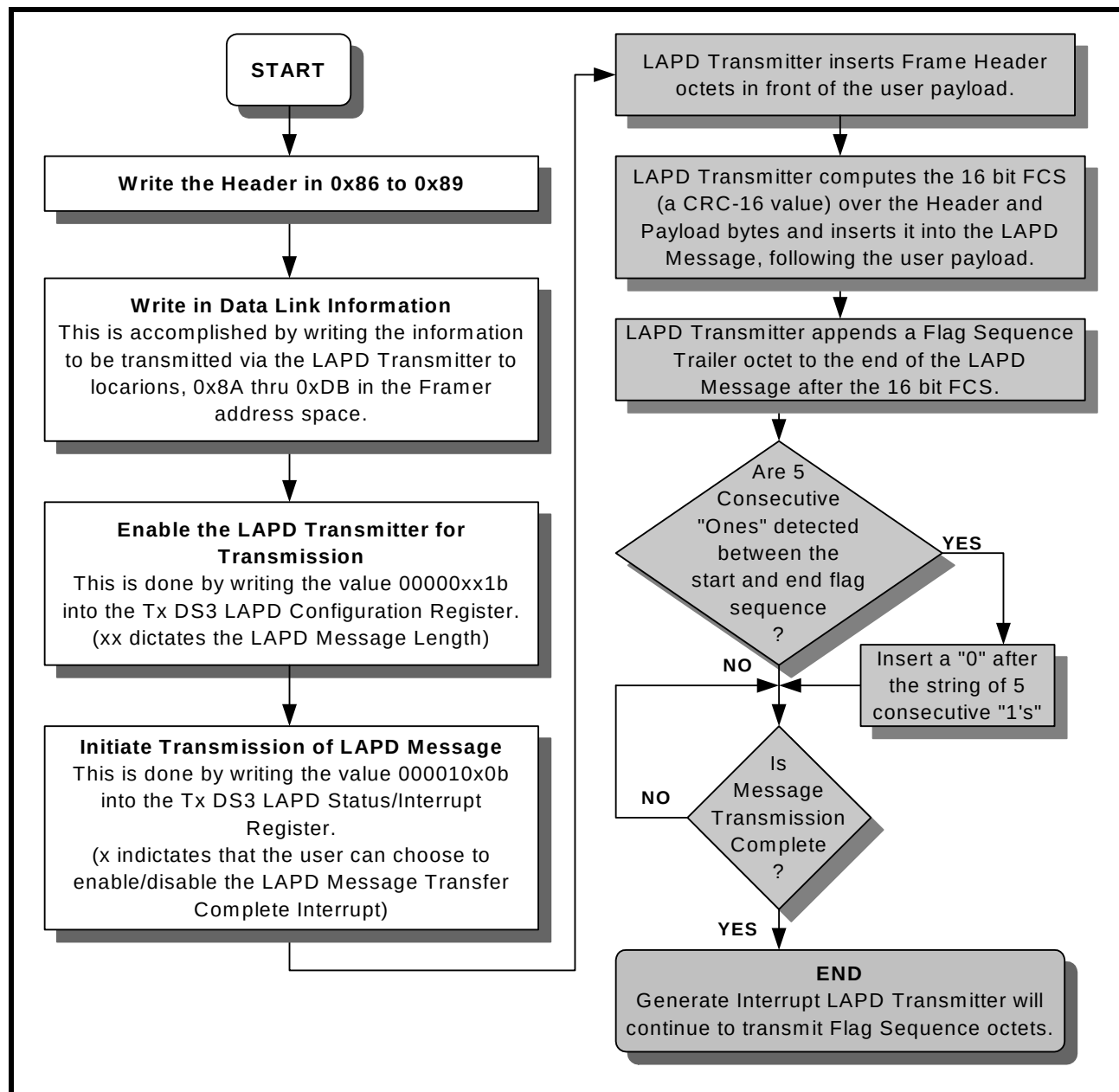
FIGURE 105. FLOW CHART DEPICTING HOW TO USE THE LAPD TRANSMITTER
