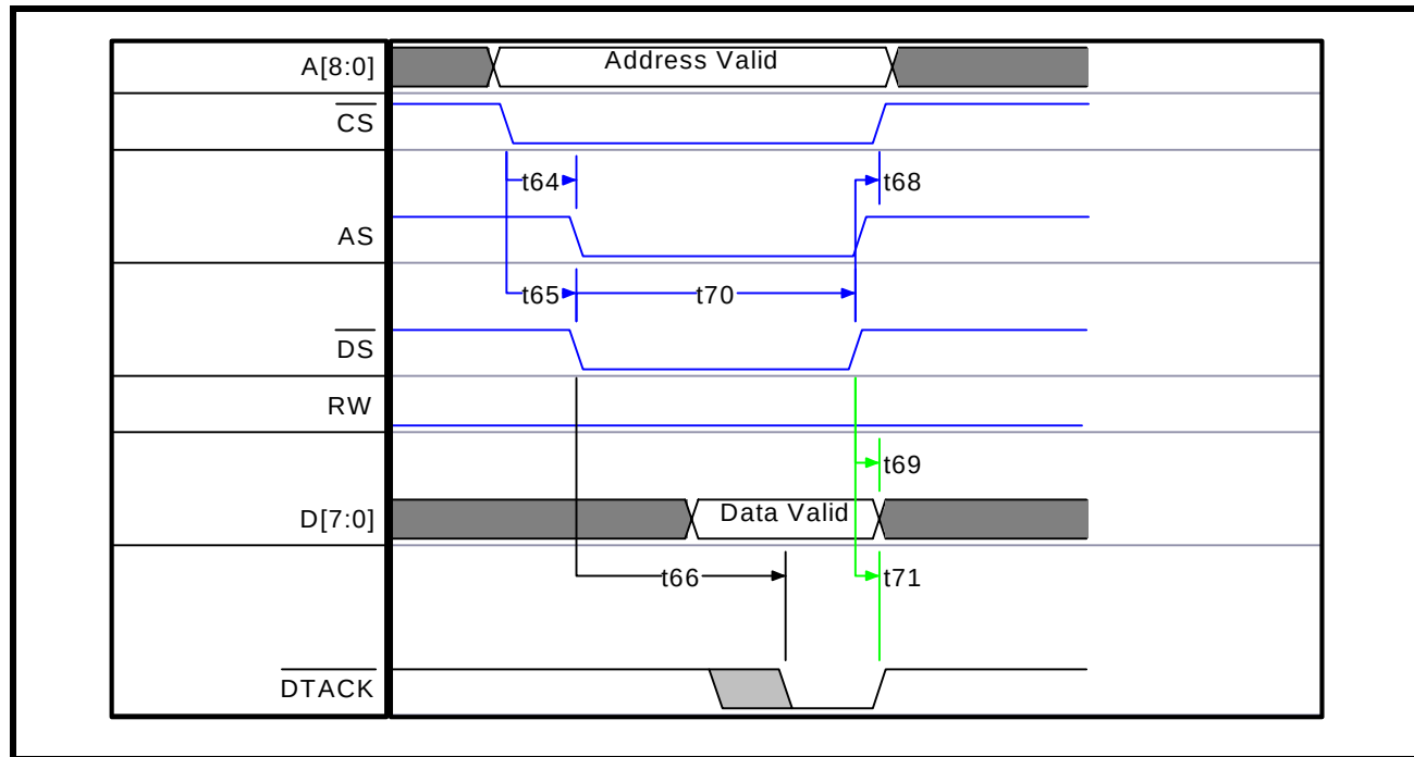
FIGURE 19. MICROPROCESSOR INTERFACE TIMING - MOTOROLA-TYPE PROGRAMMED I/O WRITE OPERATION
