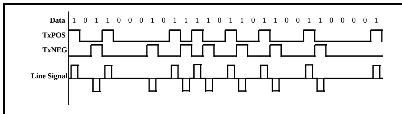
FIGURE 110. ILLUSTRATION OF AMI LINE CODE
