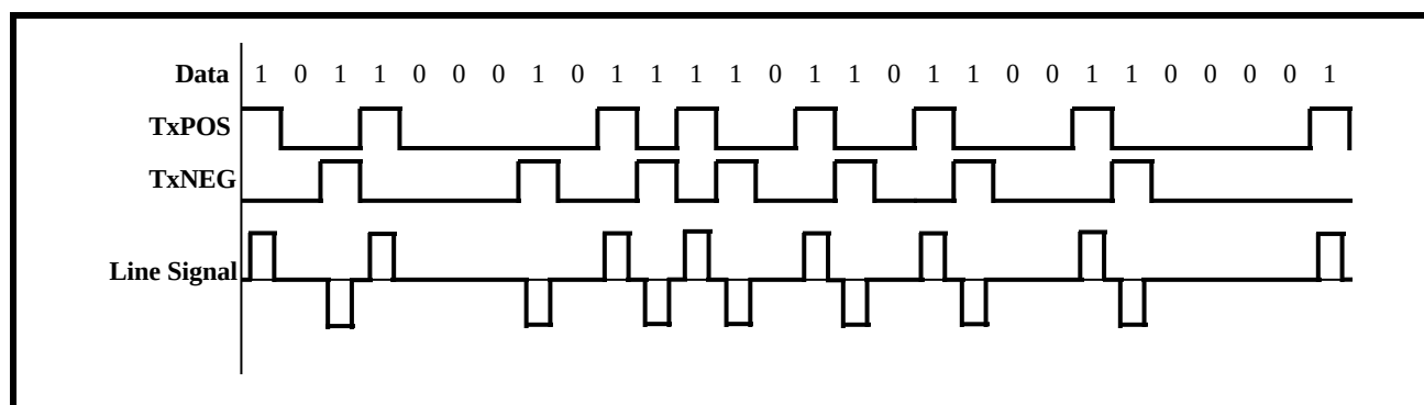
FIGURE 55. ILLUSTRATION OF AMI LINE CODE
