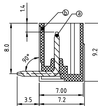
SECTION Q-Q
