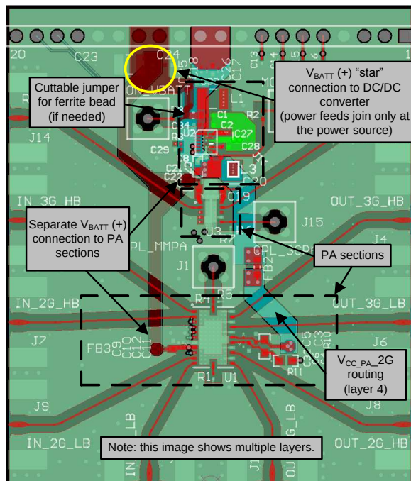
Figure 31. LM3248 V_{BATT} Star Connection and V_{CC\_PA} Routing
