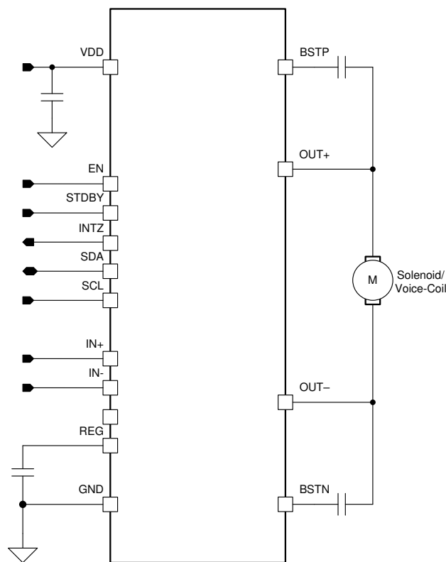
Simplified Schematic
