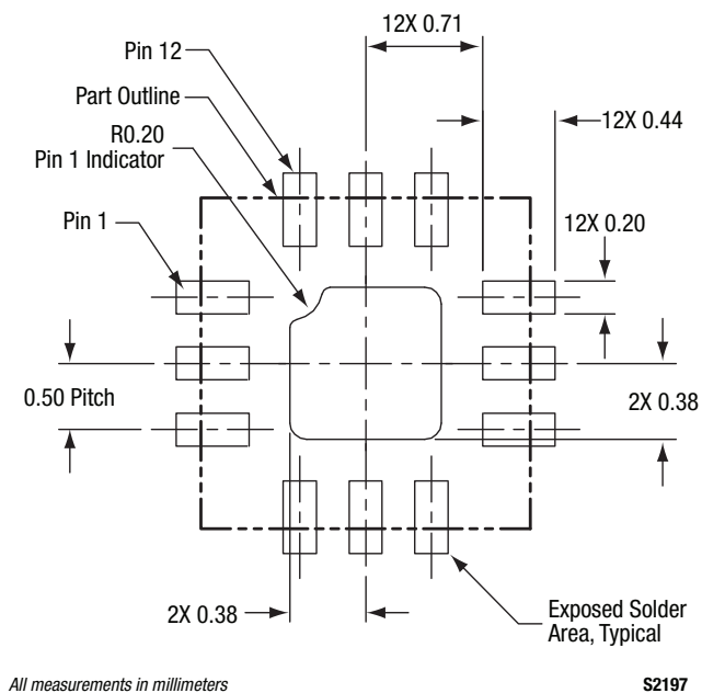
Figure 9. SKY13408-465LF PCB Layout Footprint (Top View)
