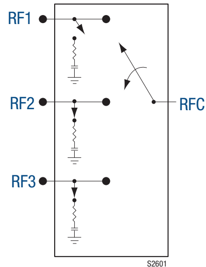
Figure 1. SKY13408-465LF Block Diagram
