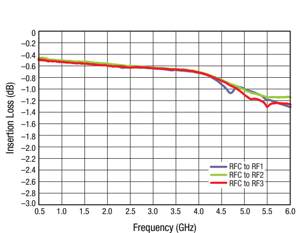
Figure 3. Typical Insertion Loss vs Frequency
