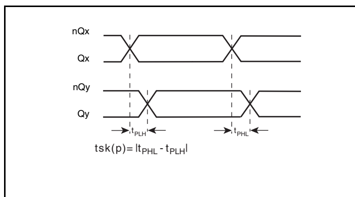
Pulse Skew
