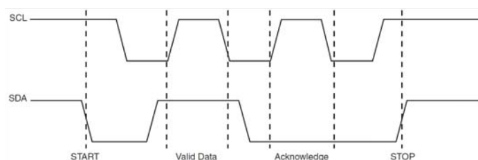
Figure 1: Standard I 2 C Transaction
