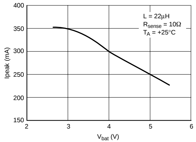
Figure 6. Typical Inductor Peak Current as a Function of V_{bat} Voltage
