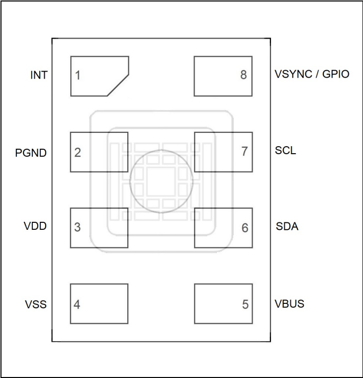
Figure 3: Pin Diagram of TCS3530
