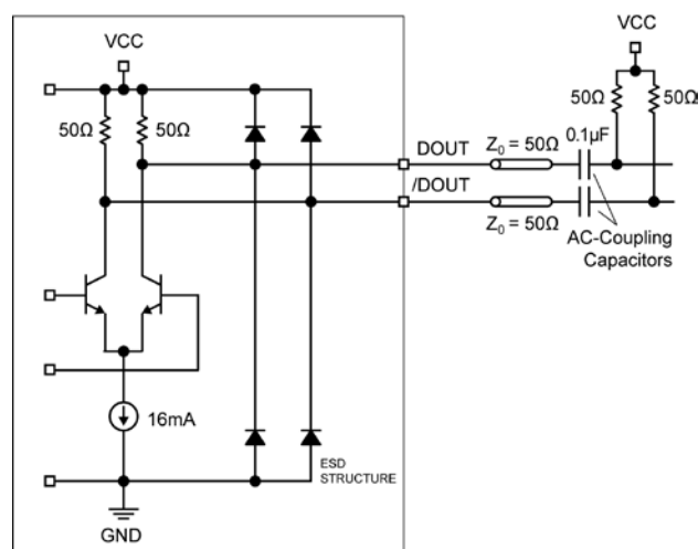
Figure 3. Output Structure
