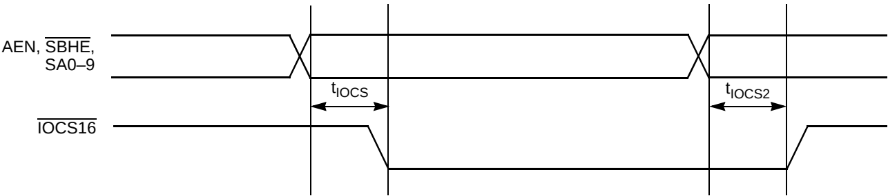
IOCS16 Timings
