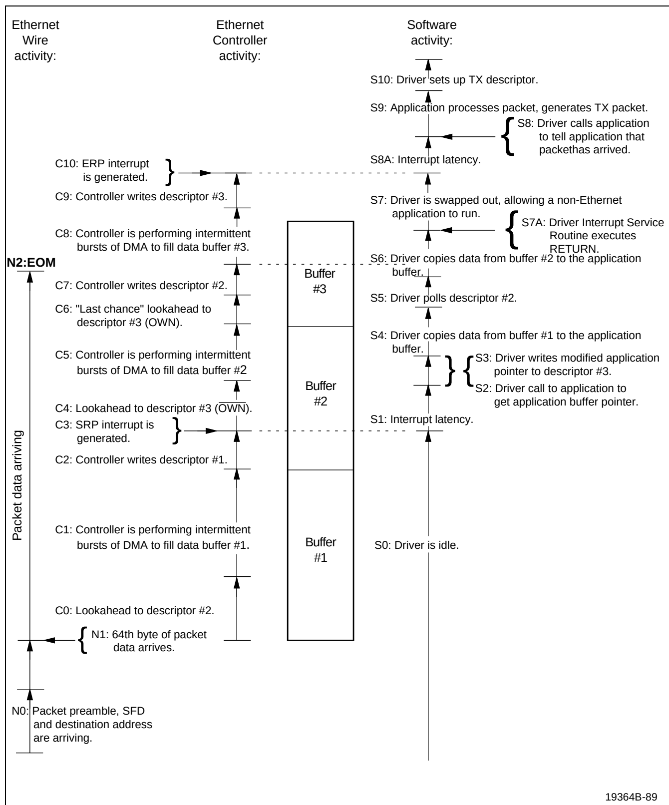
Figure 3. LAPP Timeline for TWO-INTERRUPT Method
