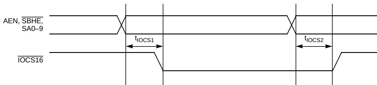
\overline{I/OCS16} Timings
