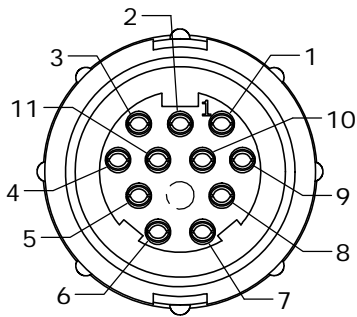
FACE VIEW W5282-11SG-3XX
