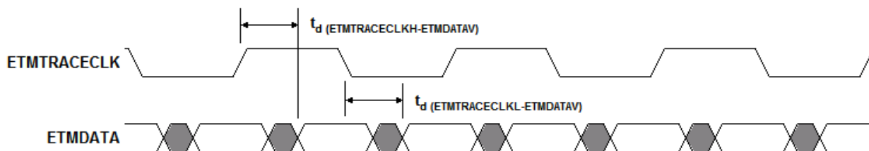
Figure 6-27. ETMDATA Timing
