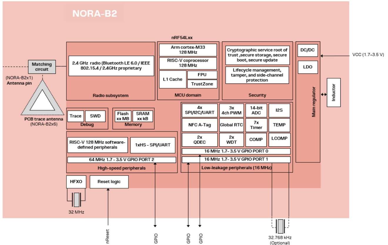
Figure 1: Block diagram of NORA-B2 series
