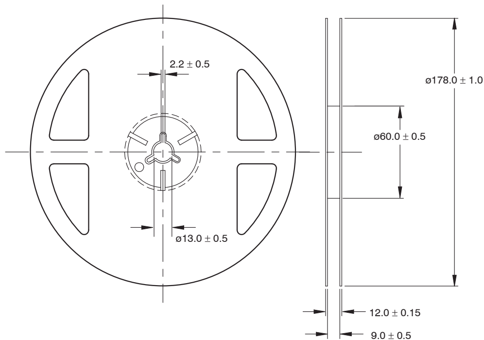
Figure 11. Reel Dimensions
