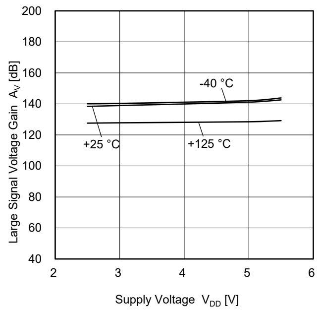
Figure 12. Large Signal Voltage Gain vs Supply Voltage ( R_L=10 k \Omega )
