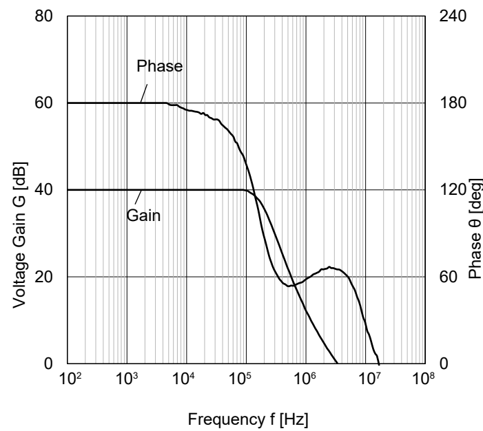
Figure 23. Voltage Gain, Phase vs Frequency ( V_{DD}=5\text{ V} )
