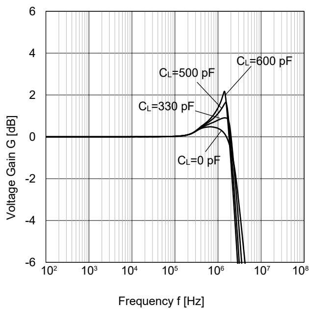
Figure 24. Voltage Gain vs Frequency ( V_{DD}=5\text{ V} , G=0\text{ dB} , V_{IN}=180\text{ mV}_{PP} )
