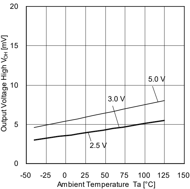
Figure 4. Output Voltage High vs Ambient Temperature (R L =10 kΩ)
