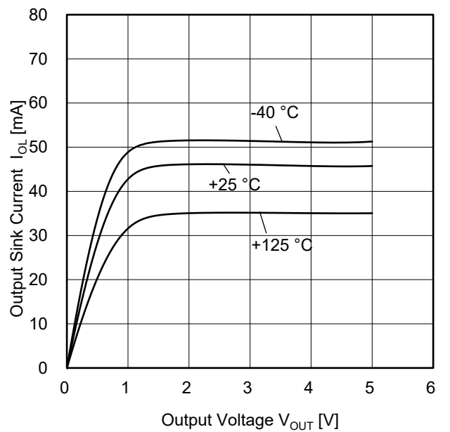
Figure 8. Output Sink Current vs Output Voltage (V DD =5 V)
