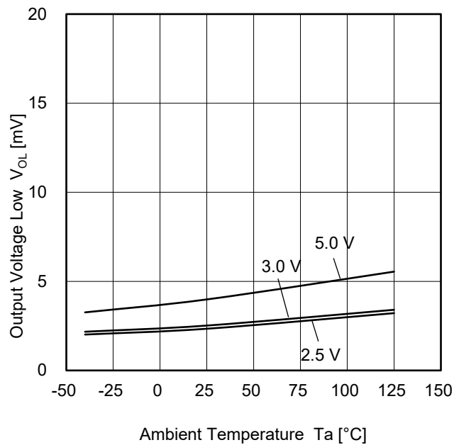
Figure 6. Output Voltage Low vs Ambient Temperature (R L =10 kΩ)
