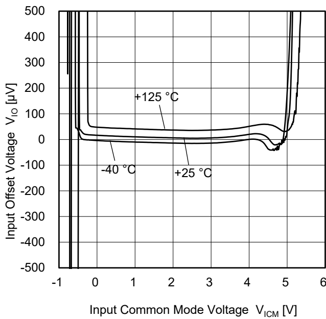
Figure 11. Input Offset Voltage vs Input Common Mode Voltage ( V_{DD}=5 V)
