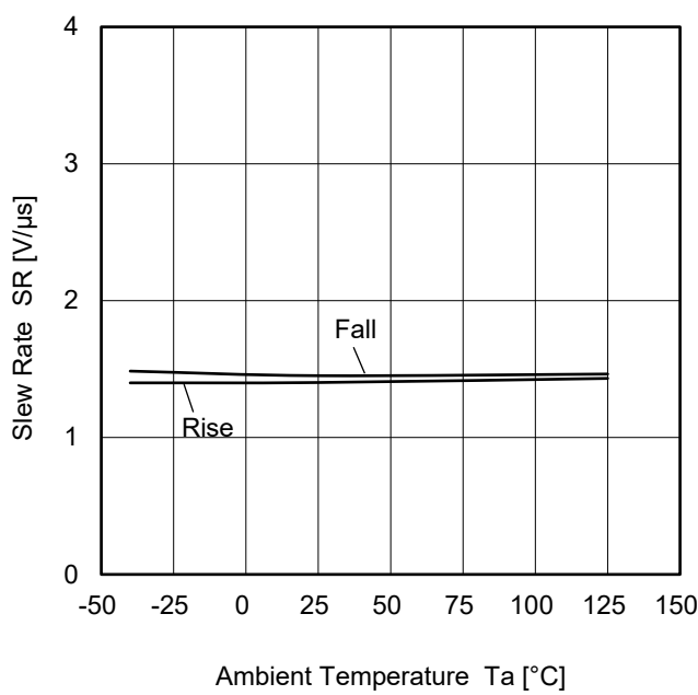
Figure 20. Slew Rate vs Ambient Temperature ( V_{DD}=5\text{ V} )
