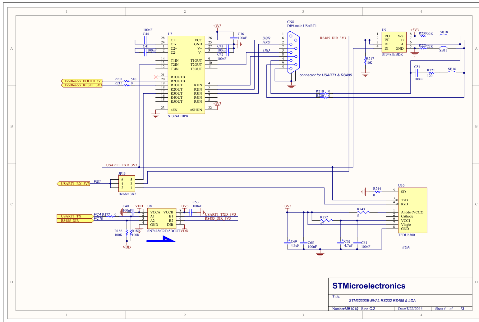
Schematics
