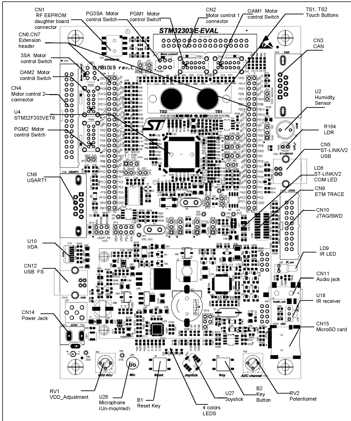
Figure 3. STM32303E-EVAL evaluation board layout
