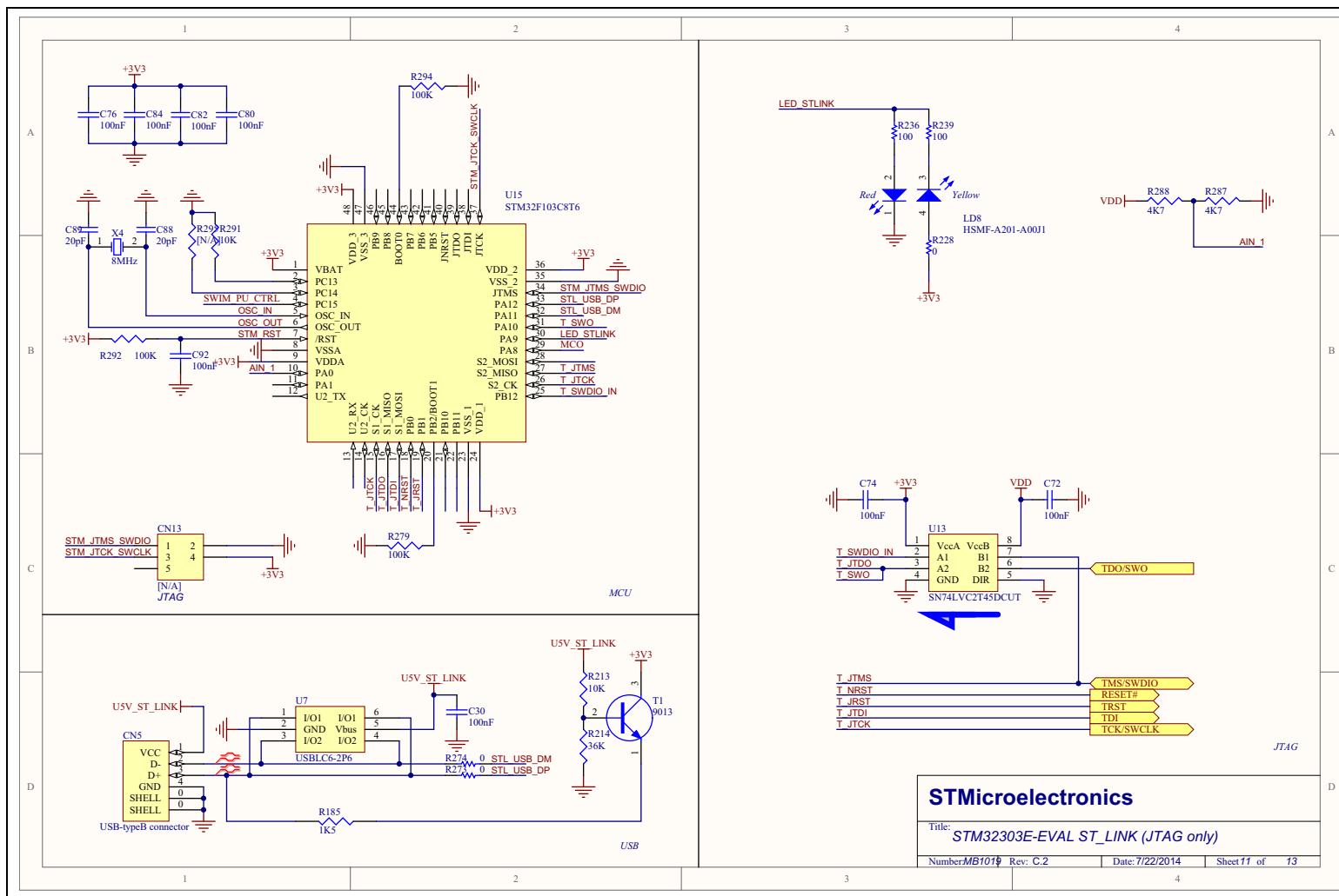
Figure 28. STM32303E-EVAL ST-LINK (JTAG only)
