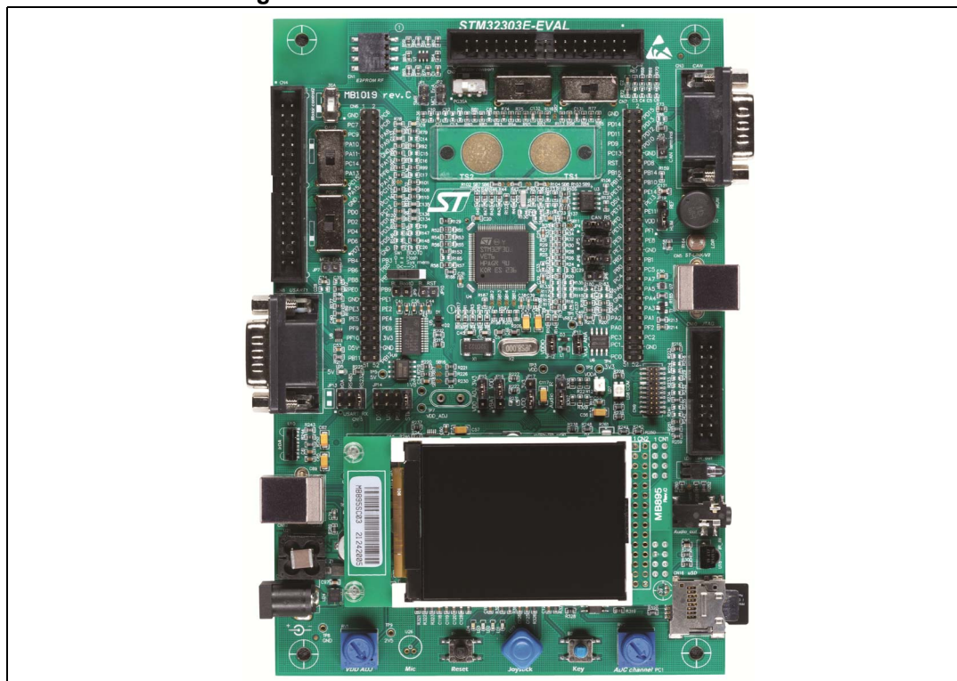
Figure 1. STM32303E-EVAL evaluation board
