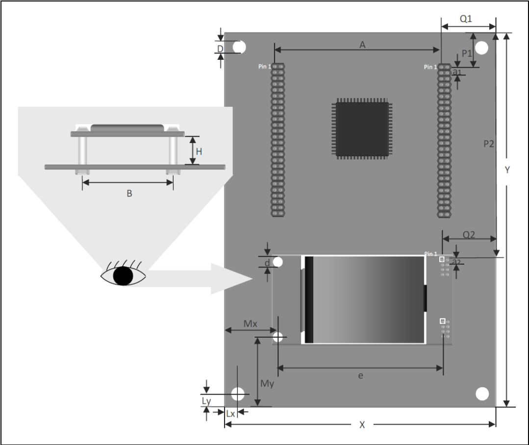
Figure 32. Mechanical dimensions
