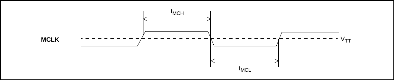
Figure 16 - Master Clock
