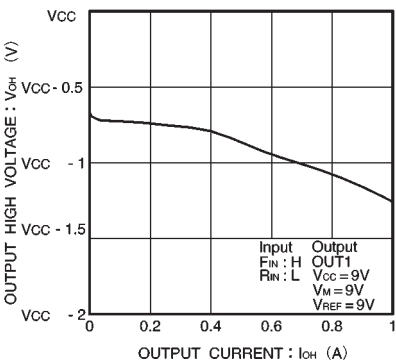
Fig.8 Output high level voltage vs. output current
