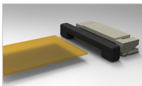
Step Three: Insert the FPC into the connector & slide stuffer backward to close
