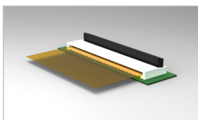
Step Three: With the FPC inserted, close the flip-lock actuator
