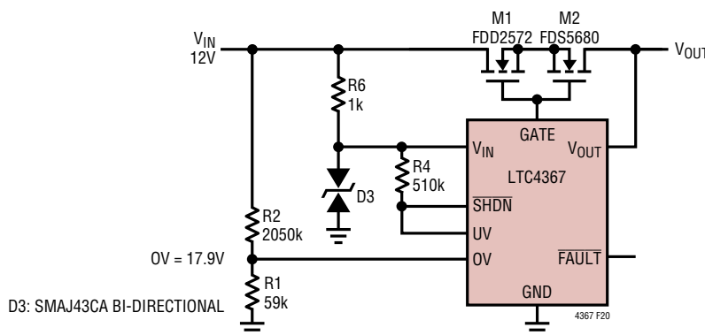
Figure 20. 12V Application Protected from 150V Transients
