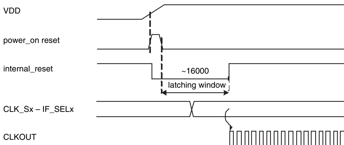
Figure 5-1. Power-on Reset
