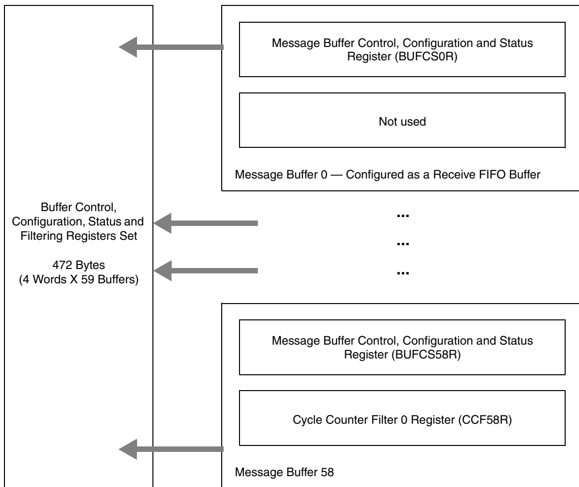
Figure 3-132. Buffer Control, Configuration, Status/Filtering Register Set for Receive FIFO Buffers
