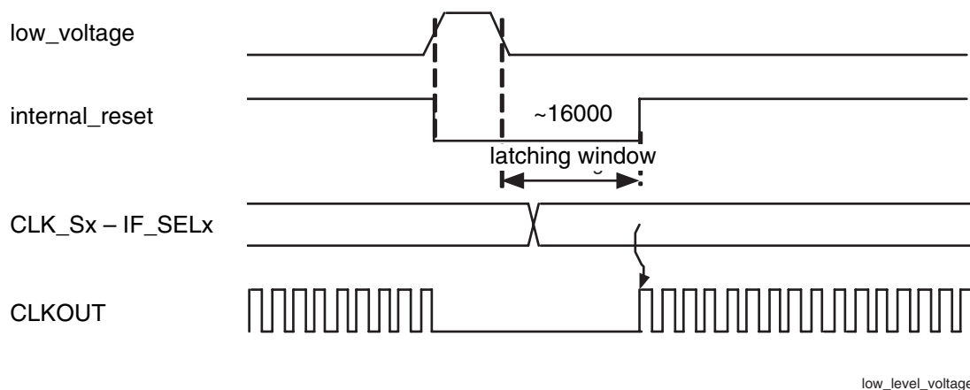
Figure 5-2. Low Voltage Reset
