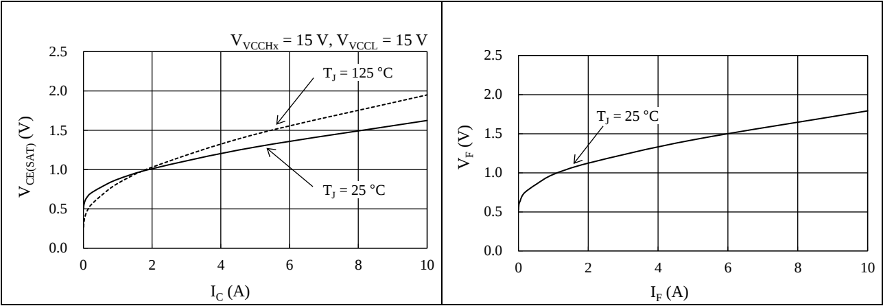
Figure 16-2. IGBT V_{CE(SAT)} vs. I_C
